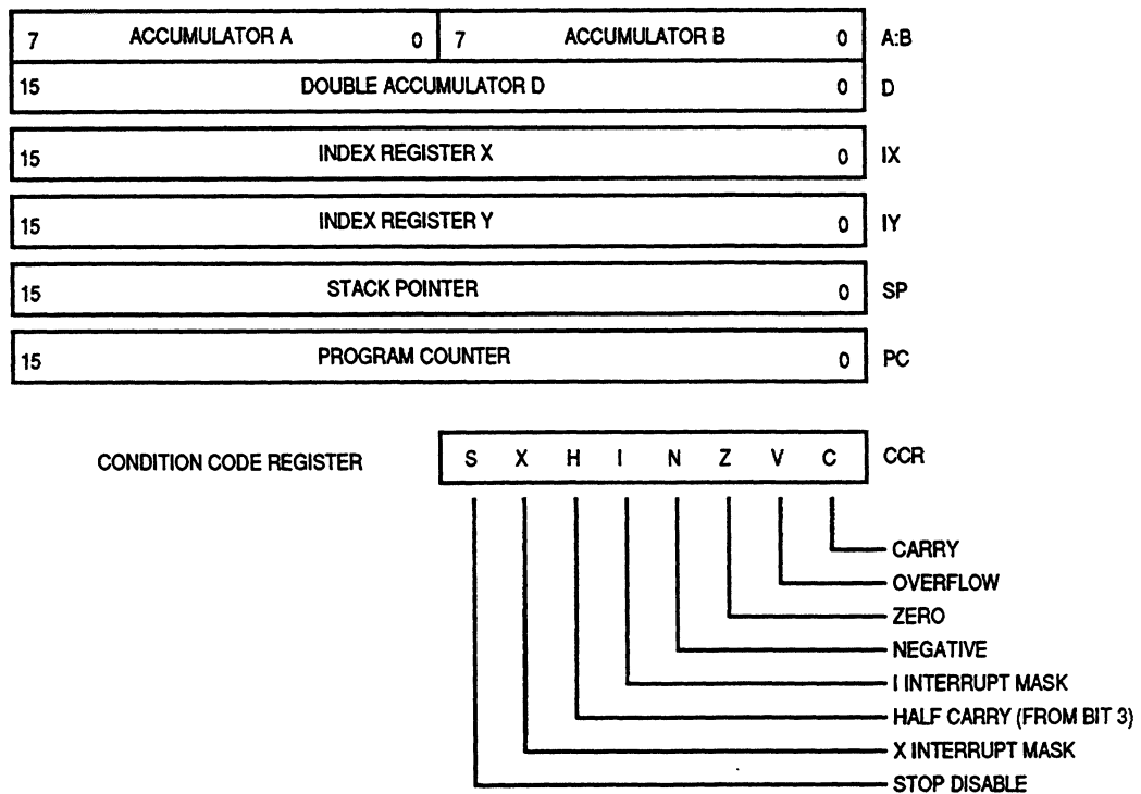
Figure 3-1. Programming Model
