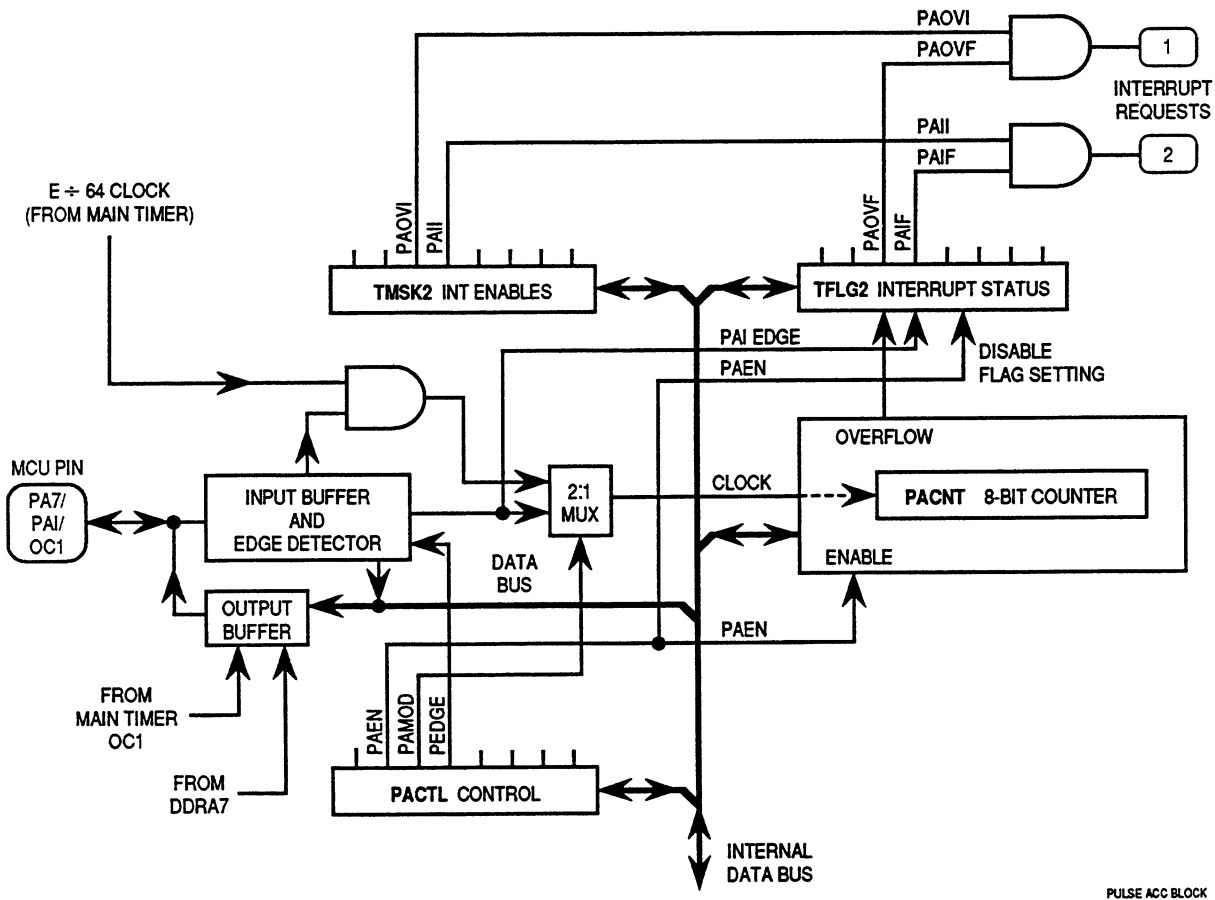
Figure 9-3. Pulse Accumulator
